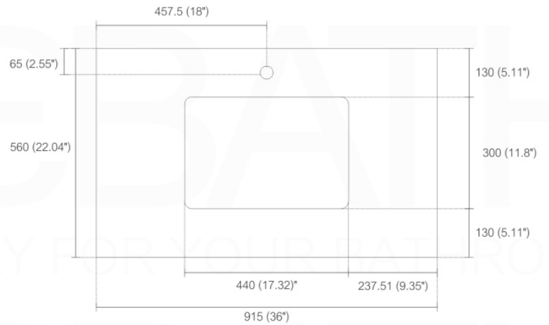
. SINK
